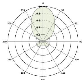
2200 Mhz E plane
